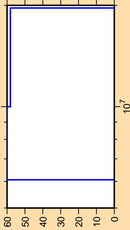
\Delta\sigma/\sigma vs. E for ^{11}\text{C}(n,ncont.)
