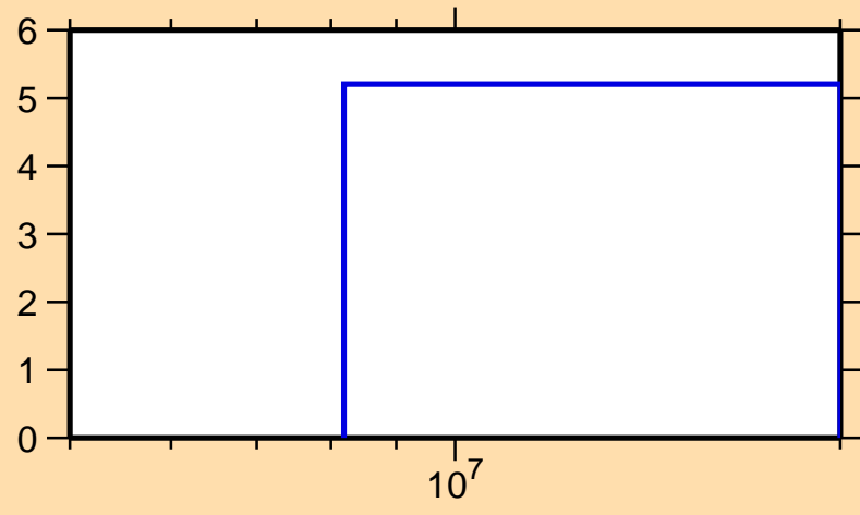
\Delta\sigma/\sigma vs. E for ^{11}\text{C}(n,n\text{onel.})
