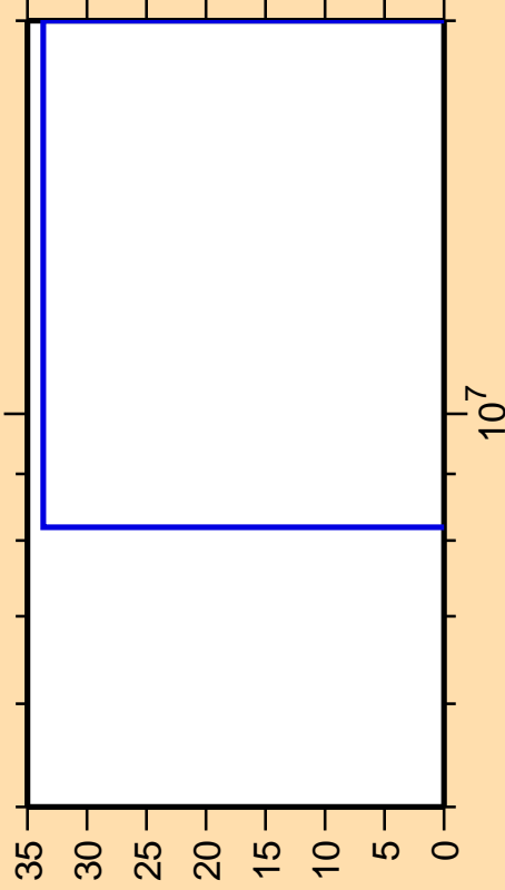
\Delta\sigma/\sigma vs. E for ^{11}\text{C}(n,p)
