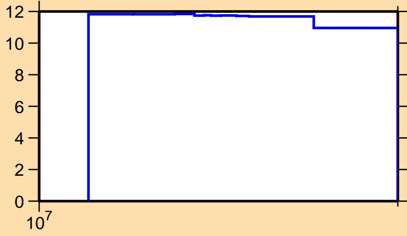
\Delta\sigma/\sigma vs. E for ^{15}\text{C}(n,el.)
