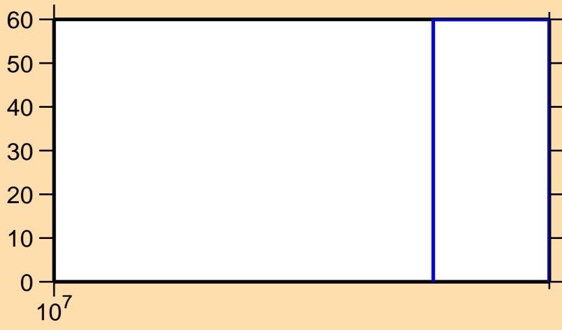
\Delta\sigma/\sigma vs. E for ^{15}\text{C}(n,ncont.)
