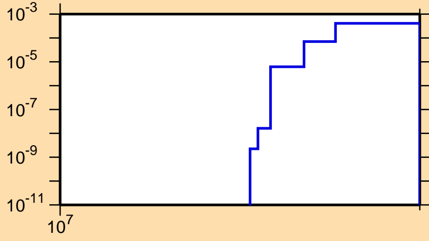
\sigma vs. E for ^{15}\text{C}(n,2n\alpha)
