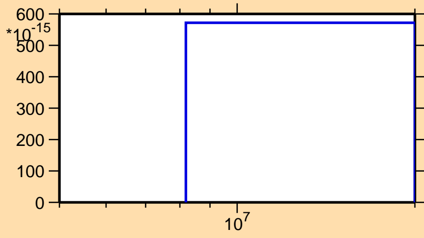
\sigma vs. E for ^{15}\text{C}(n,nt)
