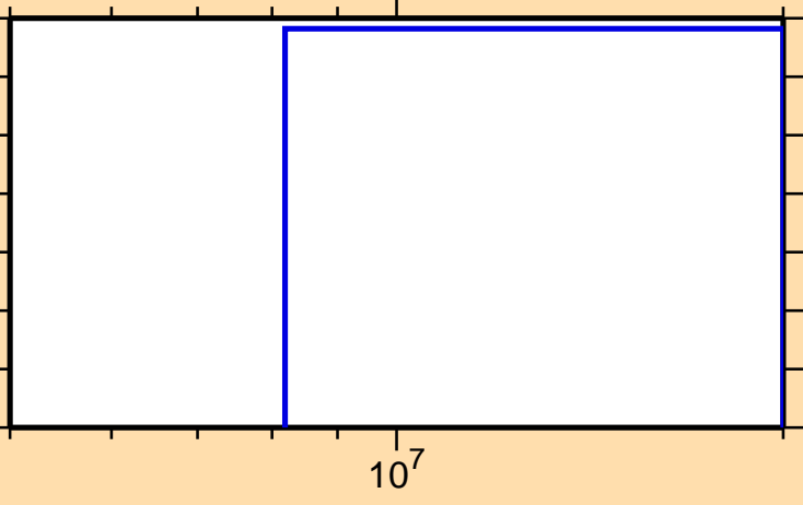
\sigma vs. E for ^{15}\text{C}(n,2n\alpha)
