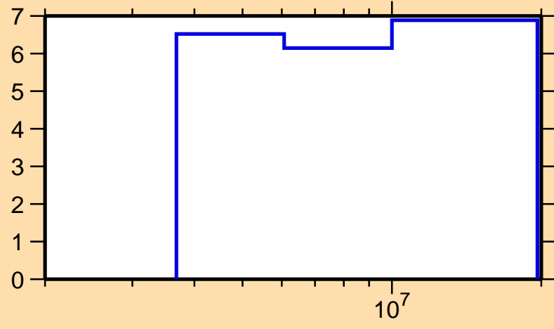
\Delta\sigma/\sigma vs. E for ^{41}\text{Ca}(n,n\text{nonel.})
