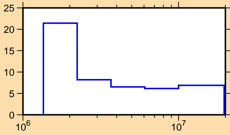
\Delta\sigma/\sigma vs. E for ^{41}\text{Ca}(n,\text{nonel.})
