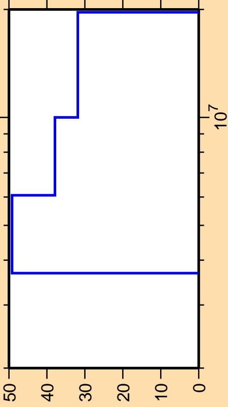
\Delta\sigma/\sigma vs. E for ^{41}\text{Ca}(n,n\text{cont.})
