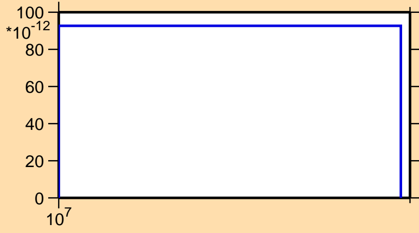
\sigma vs. E for ^{41}\text{Ca} (mt 34)
