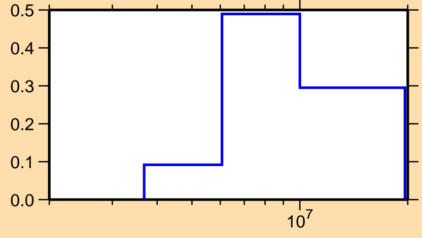
\sigma vs. E for ^{41}\text{Ca}(n,n\text{cont.})
