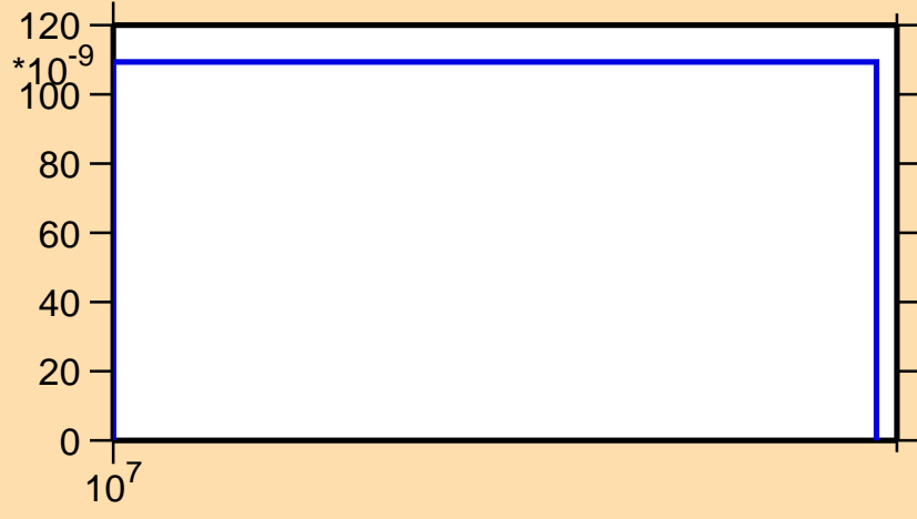
\sigma vs. E for ^{41}\text{Ca}(n,pd)
