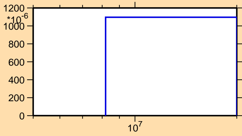
\sigma vs. E for ^{41}\text{Ca}(n,t)
