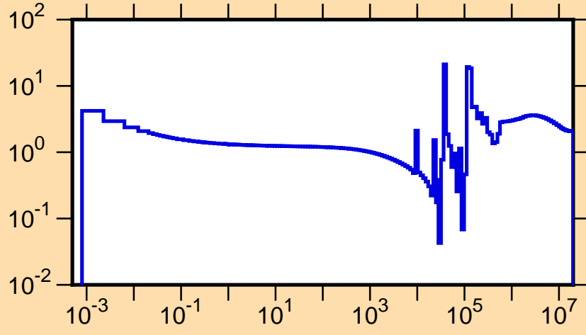
\sigma vs. E for ^{42}\text{Ca}(n,\text{tot.})
