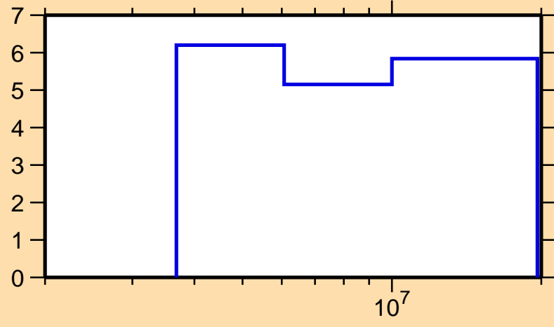
\Delta\sigma/\sigma vs. E for ^{42}\text{Ca}(n,n\text{nonel.})
