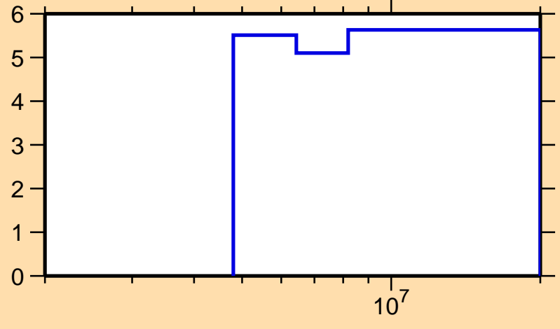
\Delta\sigma/\sigma vs. E for ^{42}\text{Ca}(n,n\text{nonel.})
