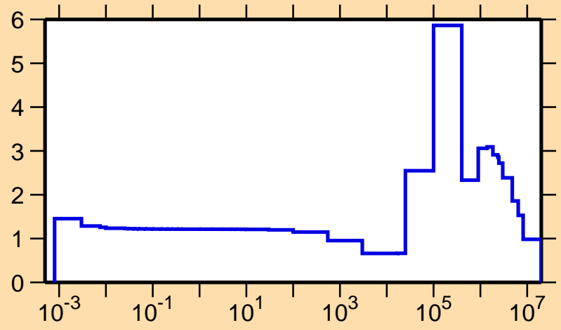
\sigma vs. E for ^{42}\text{Ca}(n,\text{el.})
