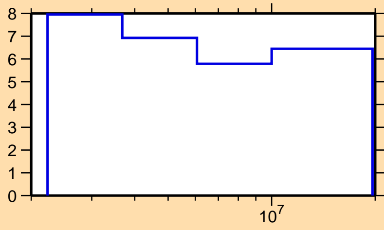
\Delta\sigma/\sigma vs. E for ^{43}\text{Ca}(n,n\text{nonel.})
