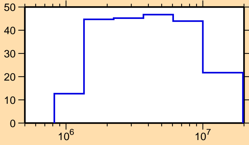
\Delta\sigma/\sigma vs. E for ^{43}\text{Ca}(n,p)
