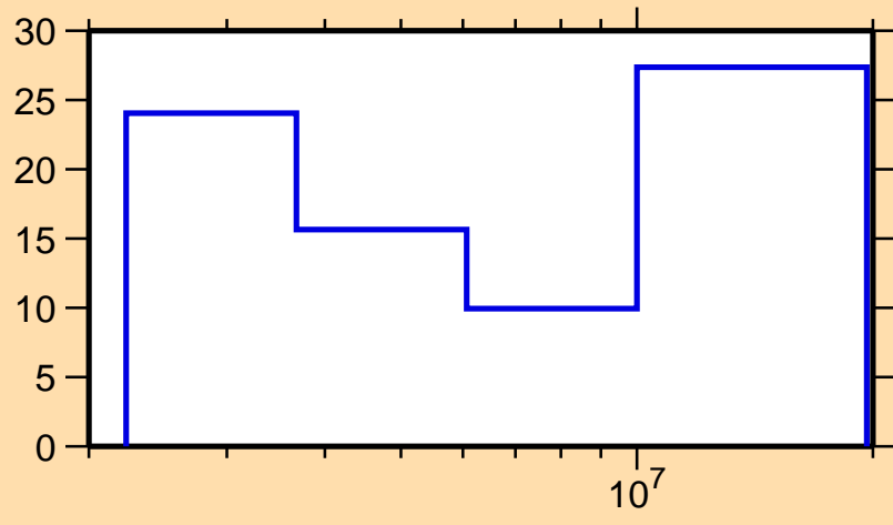
\Delta\sigma/\sigma vs. E for ^{43}\text{Ca}(n,ncont.)
