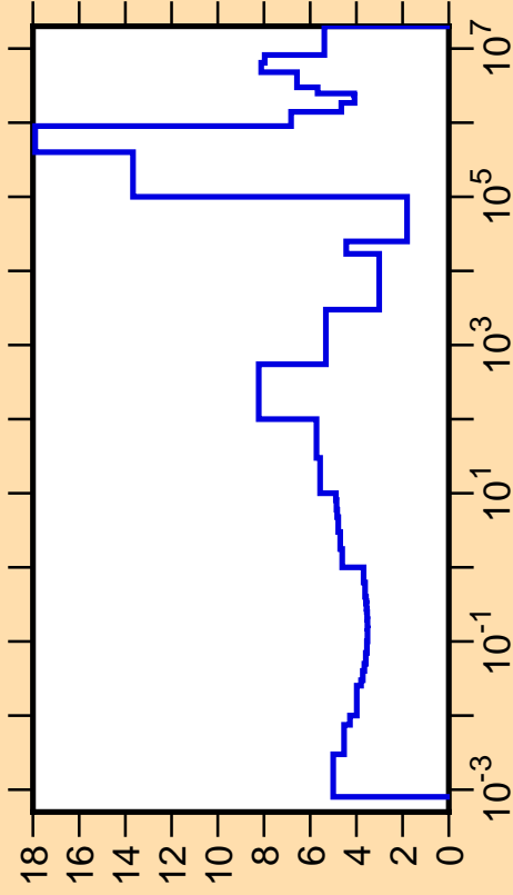
\Delta\sigma/\sigma vs. E for ^{43}\text{Ca}(n,\text{tot.})
