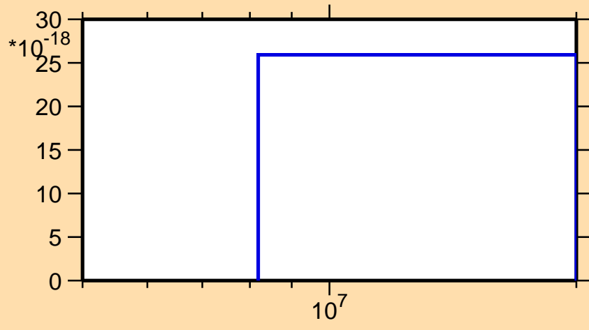
\sigma vs. E for ^{43}\text{Ca}(n,\text{pd})
