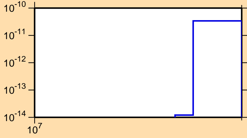
\sigma vs. E for ^{45}\text{Ca}(n,\text{He}3)
