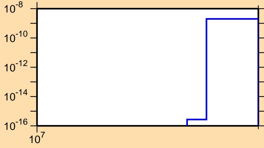
\sigma vs. E for ^{45}\text{Ca}(n,2n\alpha)
