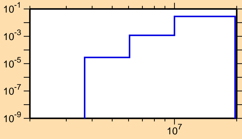
\sigma vs. E for ^{45}\text{Ca}(n,p)
