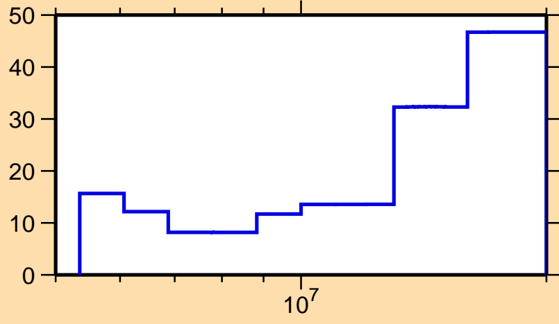
\Delta\sigma/\sigma vs. E for ^{46}\text{Ca}(n,n\text{cont.})
