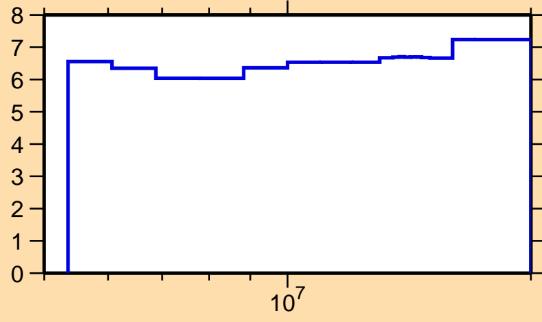
\Delta\sigma/\sigma vs. E for ^{46}\text{Ca}(n,n\text{onel.})
