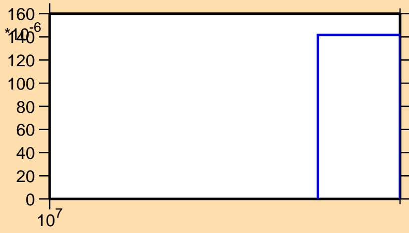
\sigma vs. E for ^{46}\text{Ca}(n,3n)
