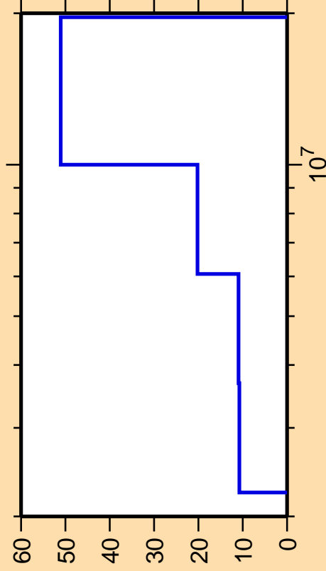
\Delta\sigma/\sigma vs. E for ^{46}\text{Ca}(n,n_2)
