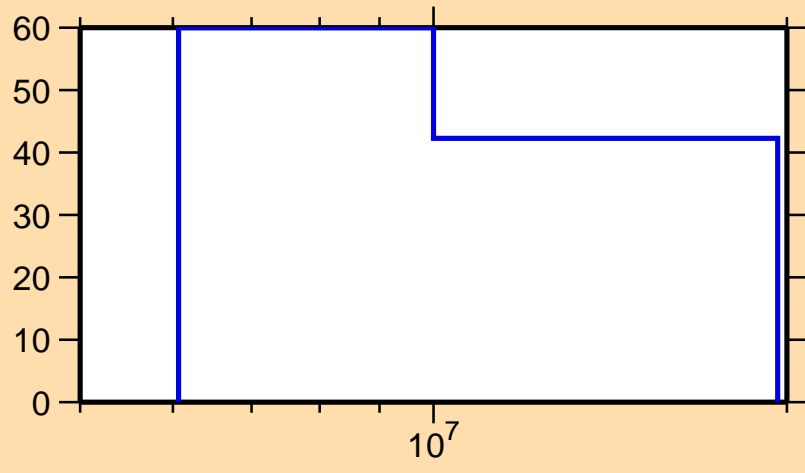
\Delta\sigma/\sigma vs. E for ^{46}\text{Ca}(n,p)
