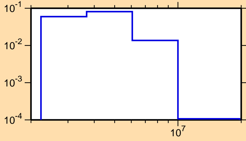
\sigma vs. E for ^{46}\text{Ca}(n,n_2)
