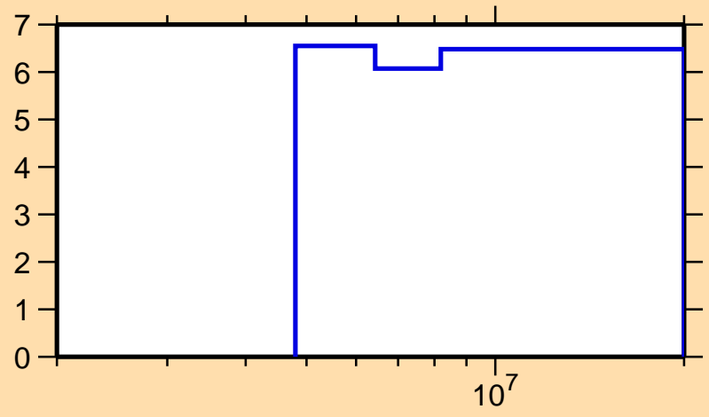
\Delta\sigma/\sigma vs. E for ^{46}\text{Ca}(n,n\text{nonel.})
