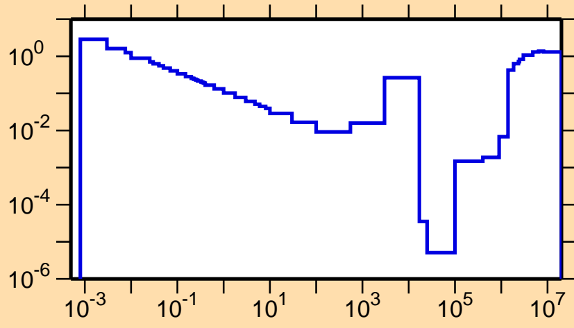
\sigma vs. E for ^{46}\text{Ca}(n,\text{nonel.})
