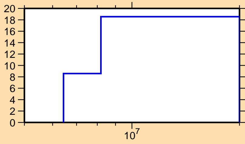
\Delta\sigma/\sigma vs. E for ^{46}\text{Ca}(n,n\text{cont.})
