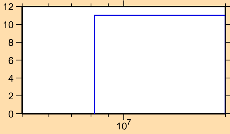
\Delta\sigma/\sigma vs. E for ^{46}\text{Ca}(n,2n)
