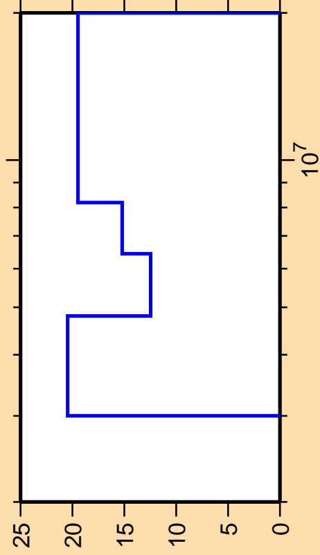
\Delta\sigma/\sigma vs. E for ^{46}\text{Ca}(n,n_4)
