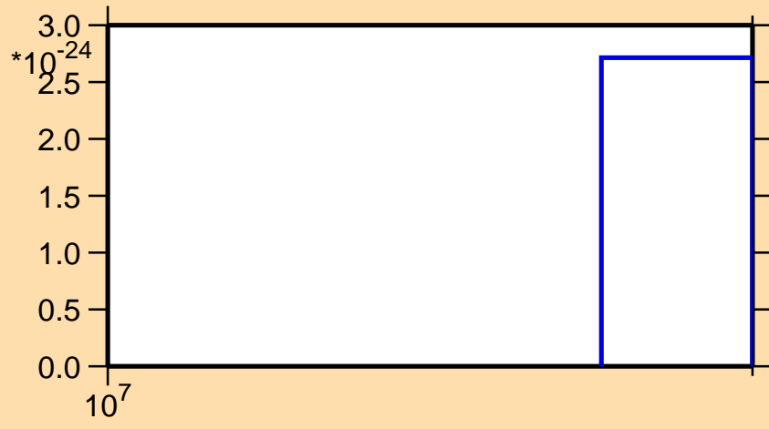
\sigma vs. E for ^{47}\text{Ca}(n,\text{He3})
