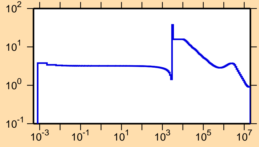
\sigma vs. E for ^{47}\text{Ca}(n,\text{el.})
