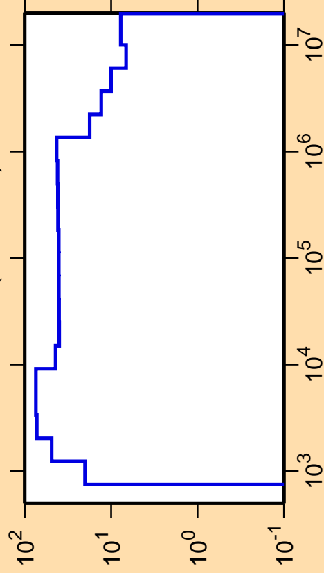
\Delta\sigma/\sigma vs. E for ^{47}\text{Ca}(n,\text{nonel.})
