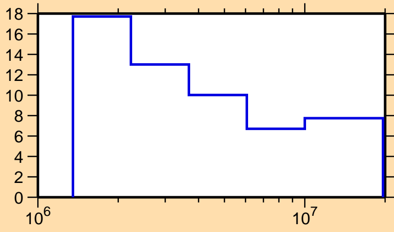
\Delta\sigma/\sigma vs. E for ^{47}\text{Ca}(n,\text{nonel.})
