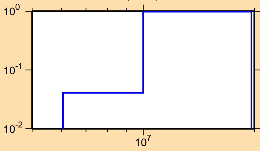
\sigma vs. E for ^{47}\text{Ca}(n,2n)
