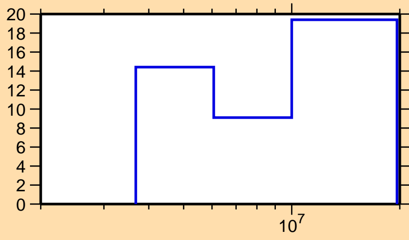
\Delta\sigma/\sigma vs. E for ^{47}\text{Ca}(n,n\text{cont.})
