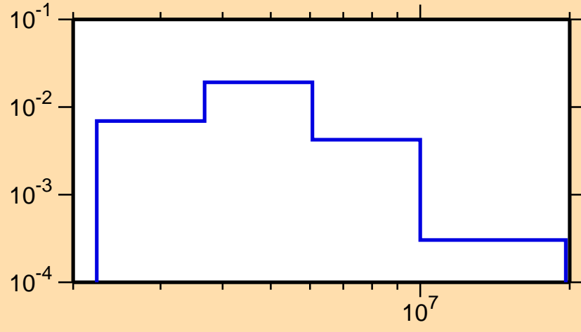
\sigma vs. E for ^{47}\text{Ca}(n,n_3)
