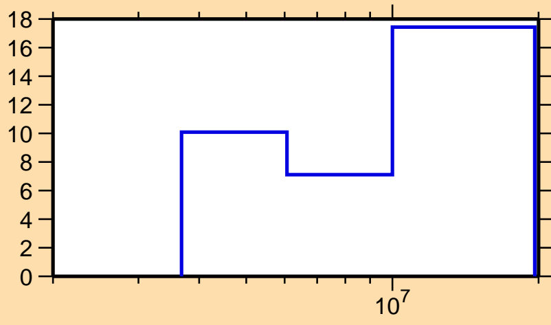
\Delta\sigma/\sigma vs. E for ^{47}\text{Ca}(n,\text{inel.})
