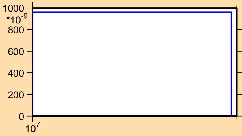
\sigma vs. E for ^{47}\text{Ca}(n,t)
