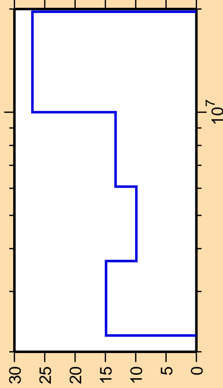
\Delta\sigma/\sigma vs. E for ^{47}\text{Ca}(n,n_4)
