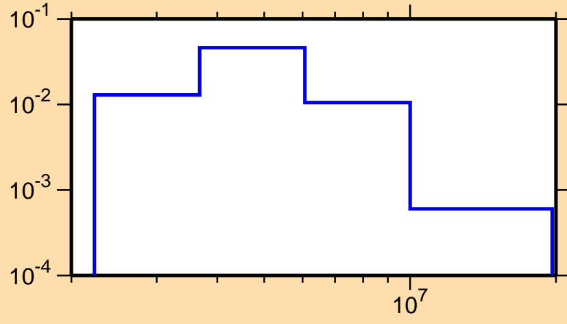
\sigma vs. E for ^{47}\text{Ca}(n,n_4)
