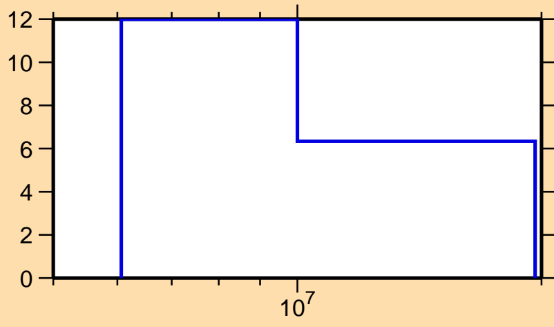
\Delta\sigma/\sigma vs. E for ^{47}\text{Ca}(n,\text{el.})
