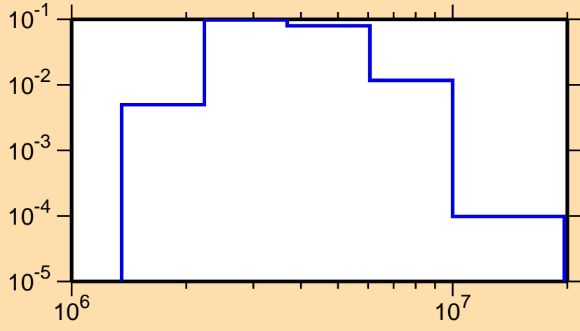
\sigma vs. E for ^{47}\text{Ca}(n,n_1)
