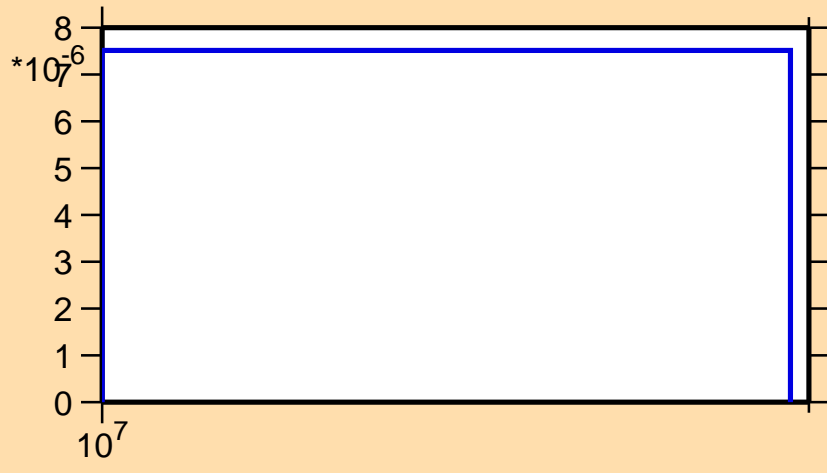
\sigma vs. E for ^{47}\text{Ca}(n,np)
