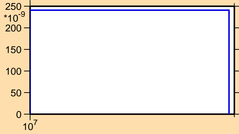
\sigma vs. E for ^{47}\text{Ca}(n,n\alpha)
