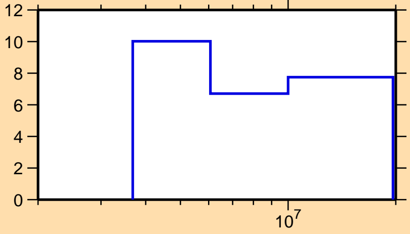
\Delta\sigma/\sigma vs. E for ^{47}\text{Ca}(n,n\text{nonel.})
