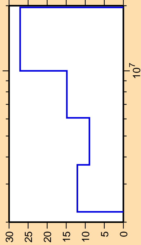
\Delta\sigma/\sigma vs. E for ^{47}\text{Ca}(n,n_3)
