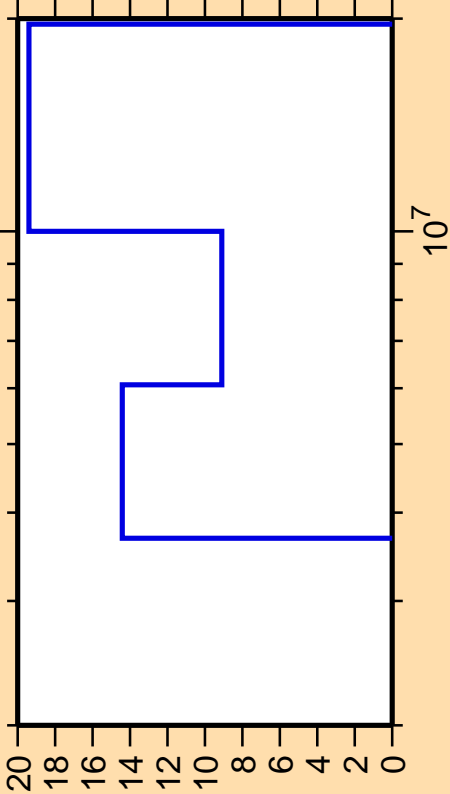
\Delta\sigma/\sigma vs. E for ^{47}\text{Ca}(n,n\text{cont.})
