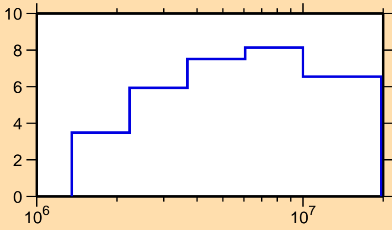
\Delta\sigma/\sigma vs. E for ^{47}\text{Ca}(n,\text{tot.})
