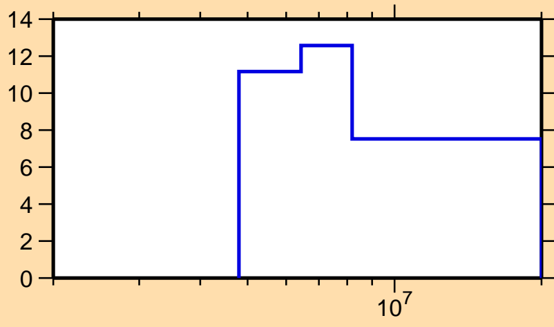
\Delta\sigma/\sigma vs. E for ^{47}\text{Ca}(n,el.)
