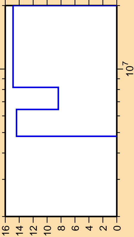
\Delta\sigma/\sigma vs. E for ^{47}\text{Ca}(n,\text{ncont.})
