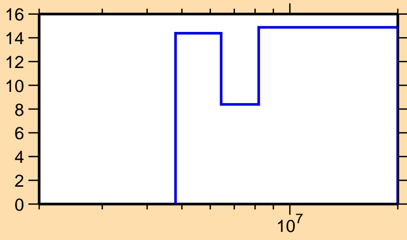
\Delta\sigma/\sigma vs. E for ^{47}\text{Ca}(n,ncont.)
