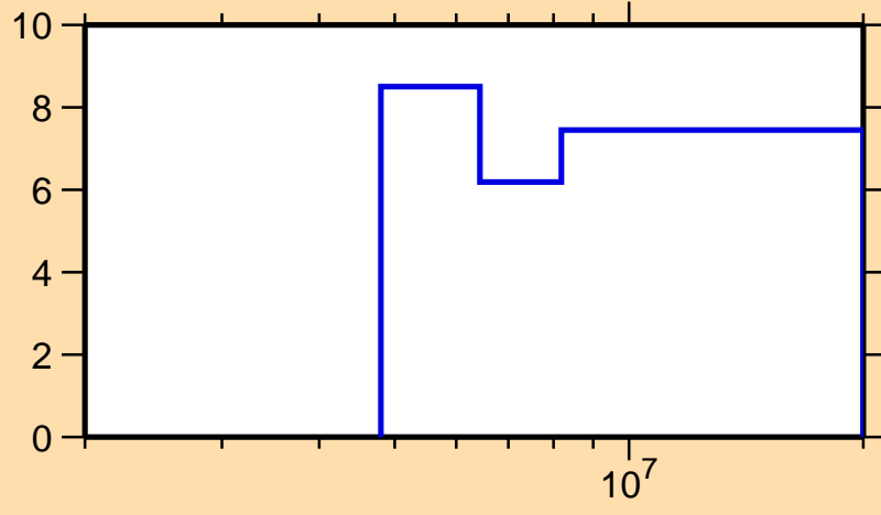
\Delta\sigma/\sigma vs. E for ^{47}\text{Ca}(n,n\text{onel.})
