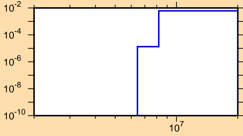
\sigma vs. E for ^{47}\text{Ca}(n,p)
