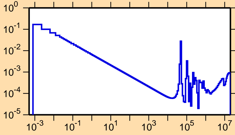
\sigma vs. E for ^{51}\text{Ca}(n,\gamma)
