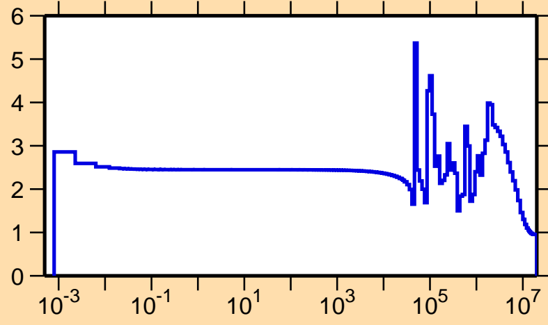
\sigma vs. E for ^{51}\text{Ca}(n,\text{el.})
