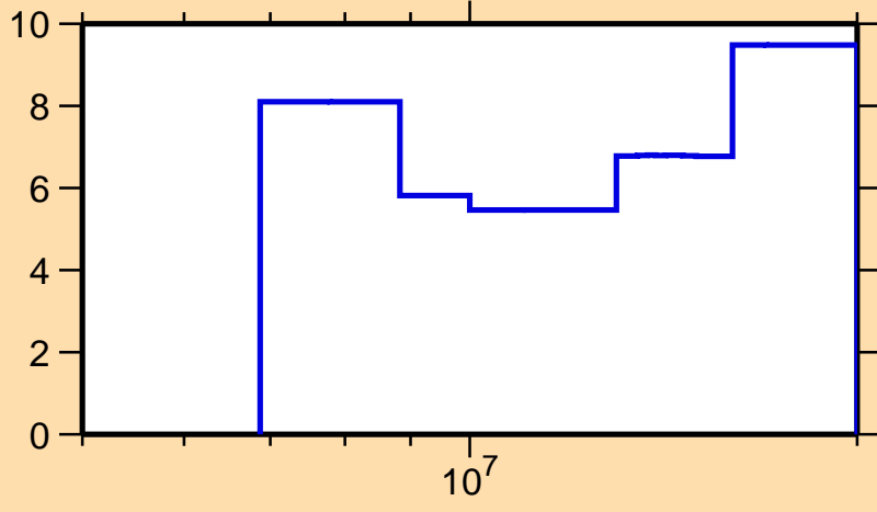
\Delta\sigma/\sigma vs. E for ^{51}\text{Ca}(n,n\text{nonel.})
