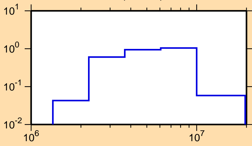
\sigma vs. E for ^{51}\text{Ca}(n,\text{inel.})
