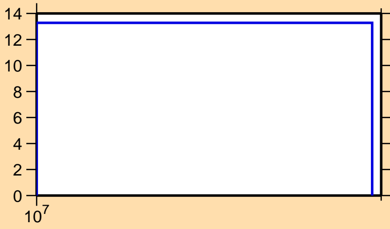
\Delta\sigma/\sigma vs. E for ^{51}\text{Ca}(n,el.)
