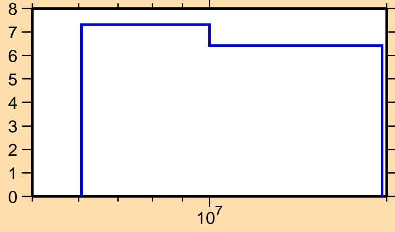
\Delta\sigma/\sigma vs. E for ^{51}\text{Ca}(n,n\text{onel.})
