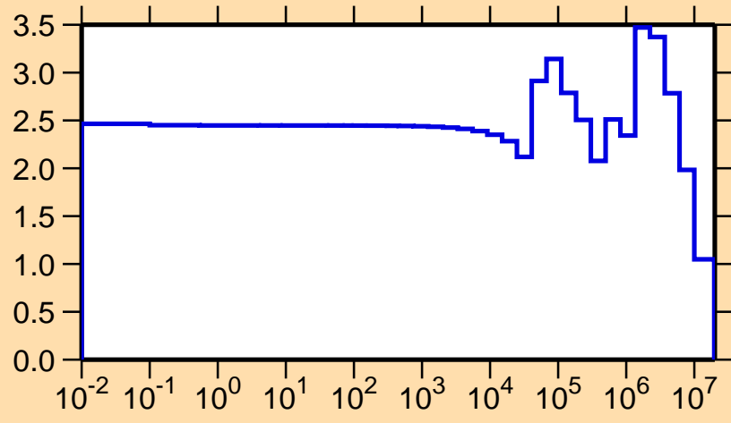
\sigma vs. E for ^{51}\text{Ca}(n,\text{el.})
