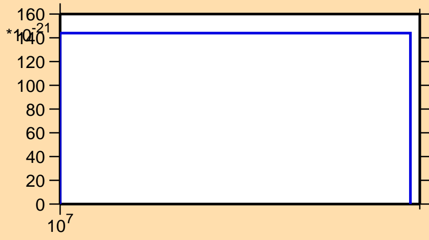
\sigma vs. E for ^{51}\text{Ca}(n,nt)
