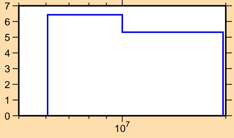
\Delta\sigma/\sigma vs. E for ^{52}\text{Ca}(n,n\text{onel.})
