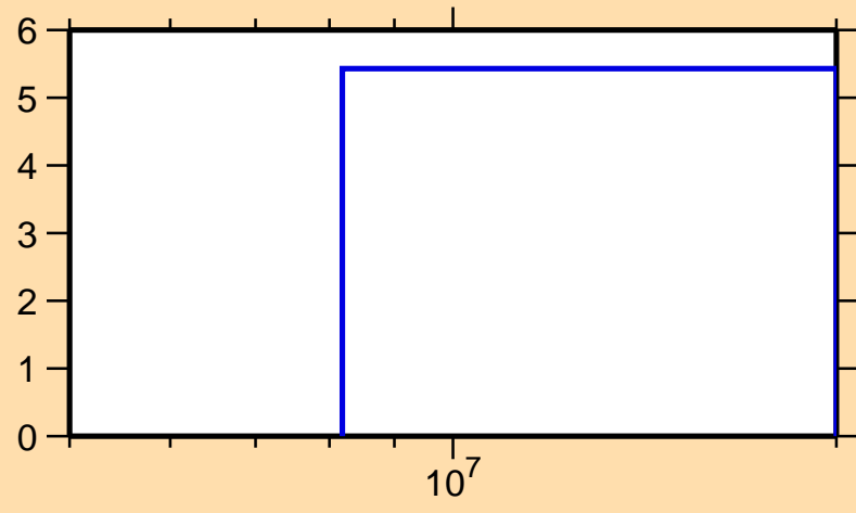
\Delta\sigma/\sigma vs. E for ^{52}\text{Ca}(n,n\text{onel.})
