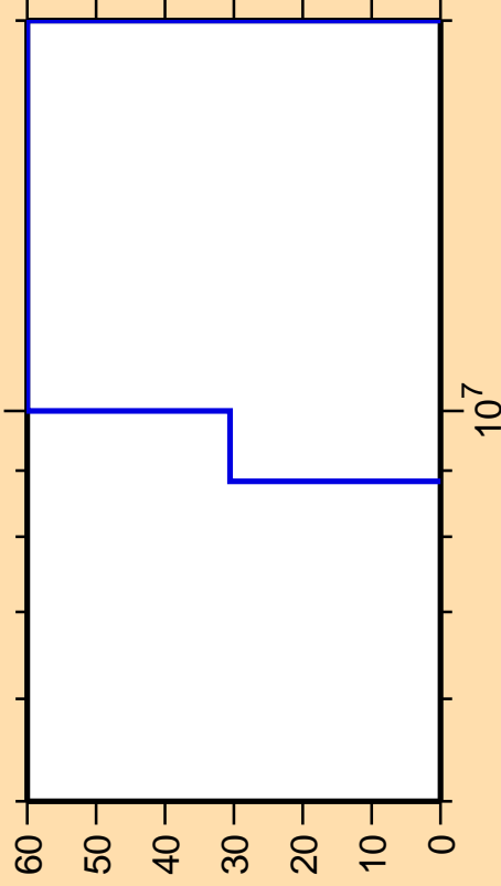
\Delta\sigma/\sigma vs. E for ^{98}\text{Cd}(n,n\alpha)
