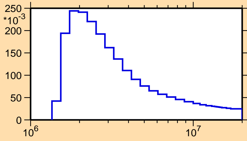
\sigma vs. E for ^{98}\text{Cd}(n,n_1)
