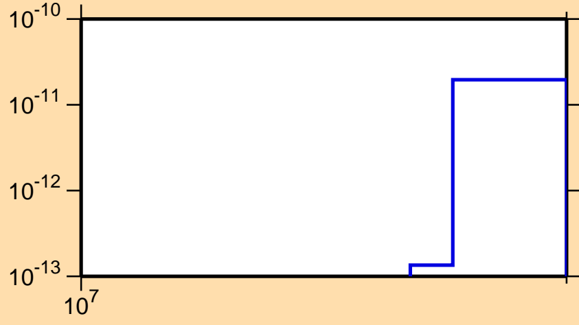
\sigma vs. E for ^{98}\text{Cd}(\text{mt117})
