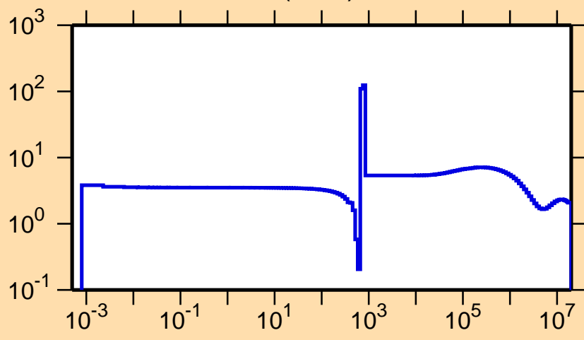
\sigma vs. E for ^{98}\text{Cd}(n,\text{el.})
