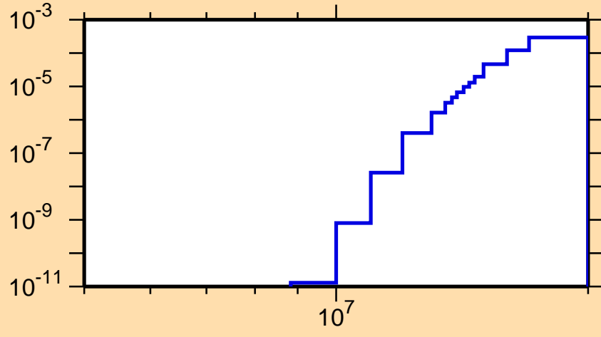
\sigma vs. E for ^{98}\text{Cd}(n,n\alpha)
