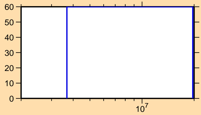
\Delta\sigma/\sigma vs. E for ^{98}\text{Cd}(n,n_1)
