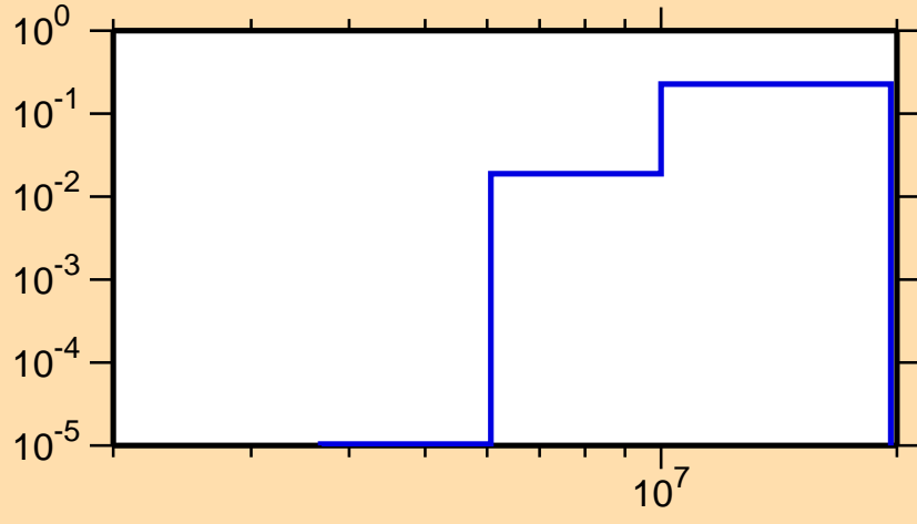
\sigma vs. E for ^{98}\text{Cd}(n,np)
