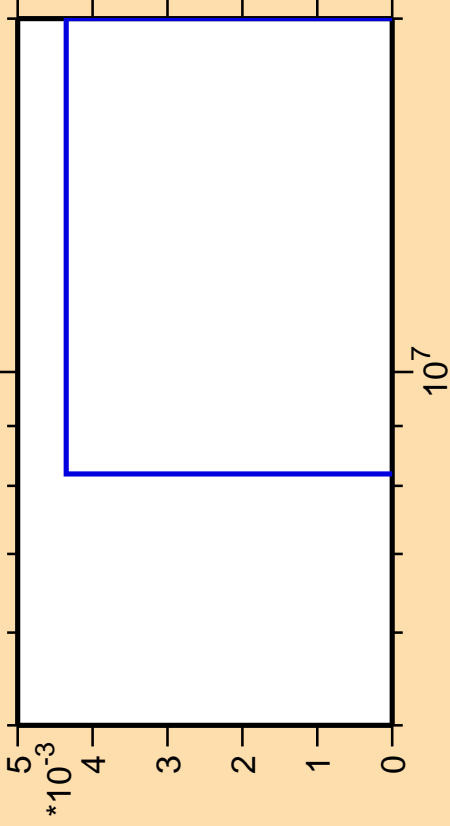
\Delta\sigma/\sigma vs. E for ^{98}\text{Cd}(n,2np)
