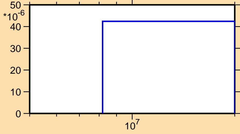
\sigma vs. E for ^{98}\text{Cd}(n,2n)
