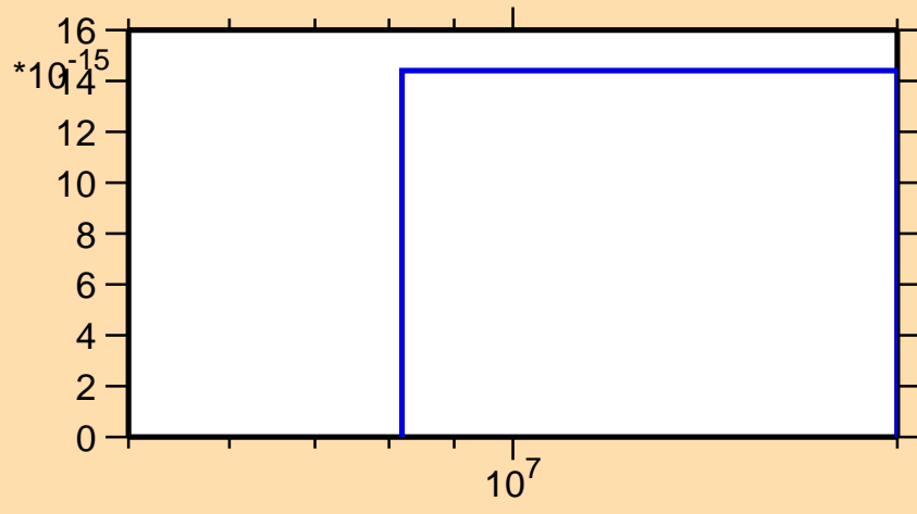
\sigma vs. E for ^{98}\text{Cd}(\text{mt } 34)
