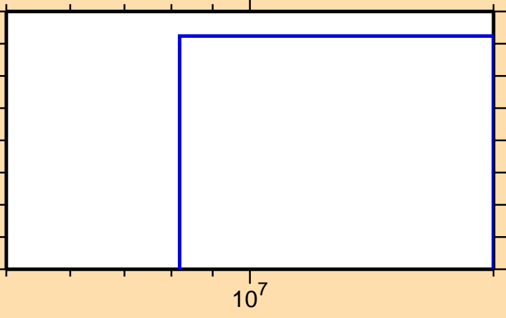
\sigma vs. E for ^{98}\text{Cd}(n,2np)
