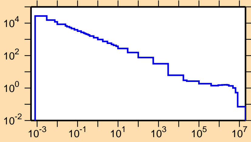
\sigma vs. E for ^{98}\text{Cd}(n,p)
