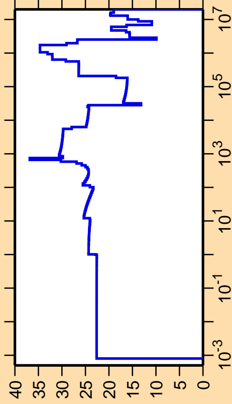
\Delta\sigma/\sigma vs. E for ^{99}\text{Cd}(n,\text{el.})
