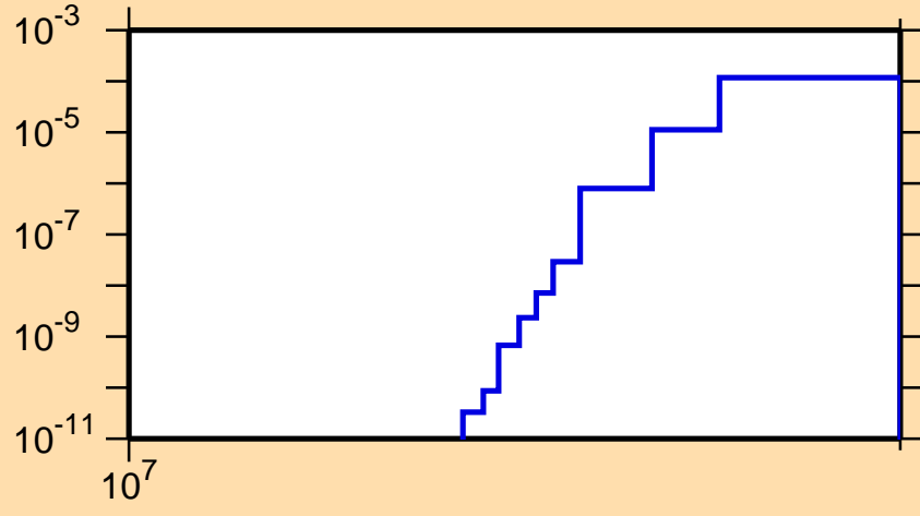
\sigma vs. E for ^{99}\text{Cd}(n,\text{pt})
