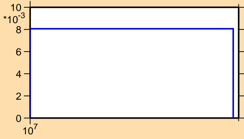
\sigma vs. E for ^{99}\text{Cd}(n,2n)
