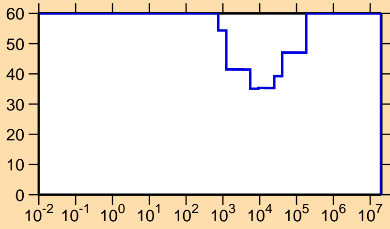
\Delta\sigma/\sigma vs. E for ^{99}\text{Cd}(n,\gamma)
