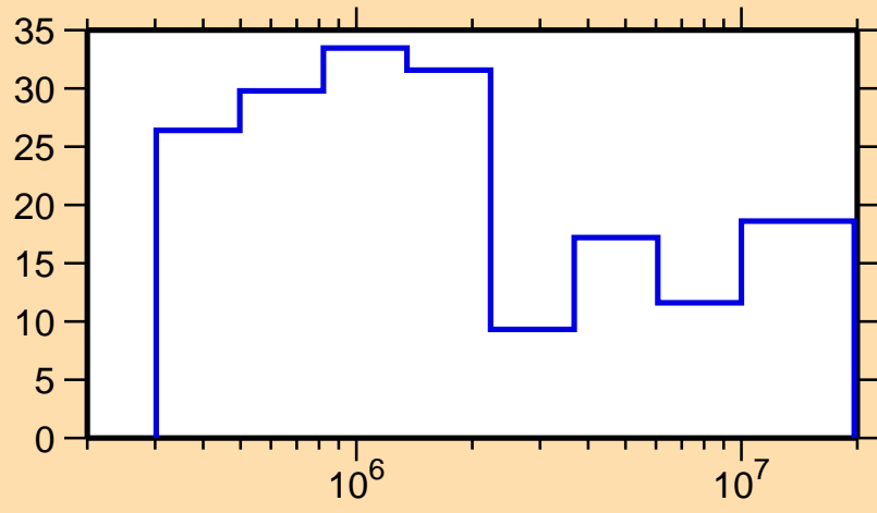
\Delta\sigma/\sigma vs. E for ^{99}\text{Cd}(n,\text{el.})
