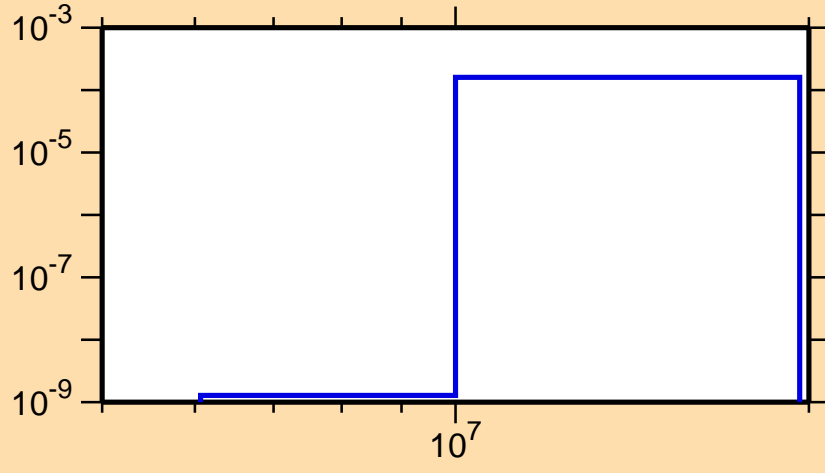
\sigma vs. E for ^{99}\text{Cd}(n,n\alpha)
