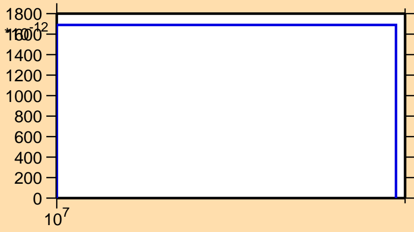
\sigma vs. E for ^{99}\text{Cd}(\text{mt } 34)
