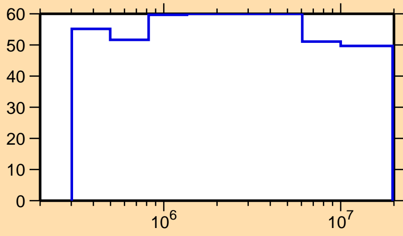
\Delta\sigma/\sigma vs. E for ^{99}\text{Cd}(n,\text{inel.})
