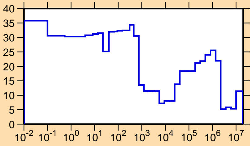
\Delta\sigma/\sigma vs. E for ^{99}\text{Cd}(n,\text{tot.})
