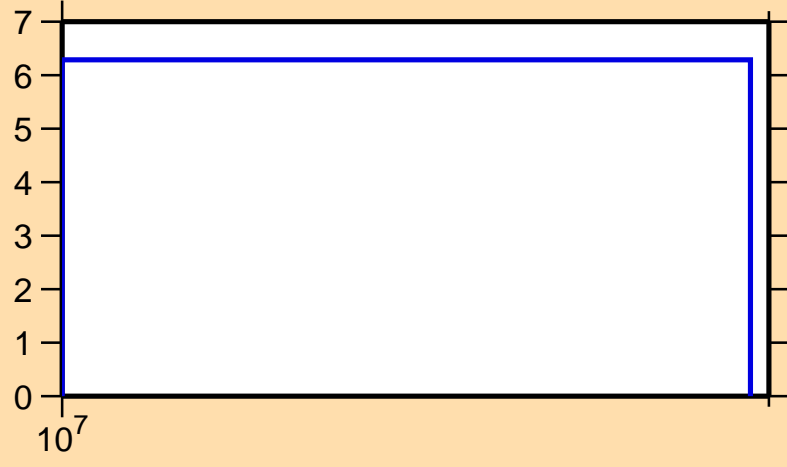
\Delta\sigma/\sigma vs. E for ^{99}\text{Cd}(n,\text{nonel.})
