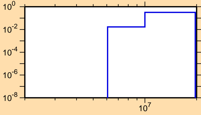
\sigma vs. E for ^{99}\text{Cd}(n,np)
