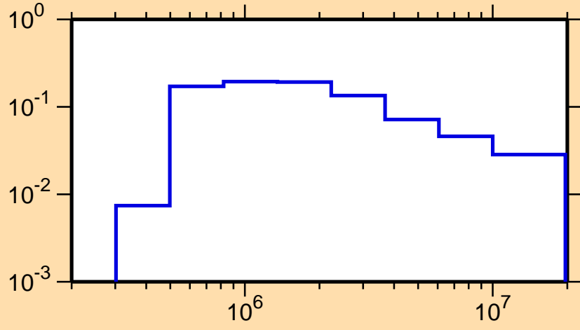
\sigma vs. E for ^{99}\text{Cd}(n,\text{inel.})
