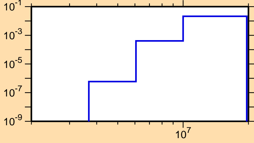
\sigma vs. E for ^{99}\text{Cd}(n,d)
