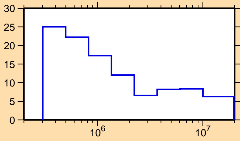
\Delta\sigma/\sigma vs. E for ^{99}\text{Cd}(n,\text{nonel.})
