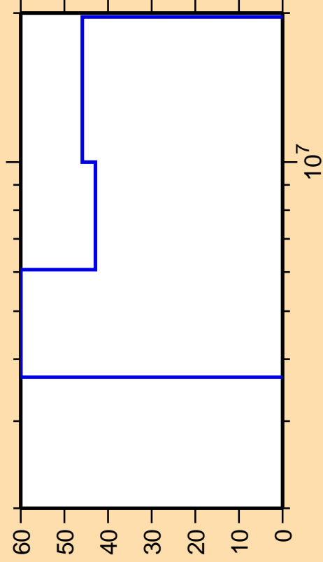
\Delta\sigma/\sigma vs. E for ^{99}\text{Cd}(n,np)
