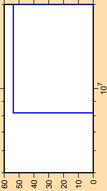
\Delta\sigma/\sigma vs. E for ^{99}\text{Cd}(\text{mt117})
