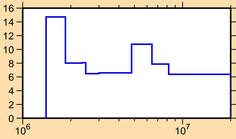
\Delta\sigma/\sigma vs. E for ^{99}\text{Cd}(n,n\text{onel.})
