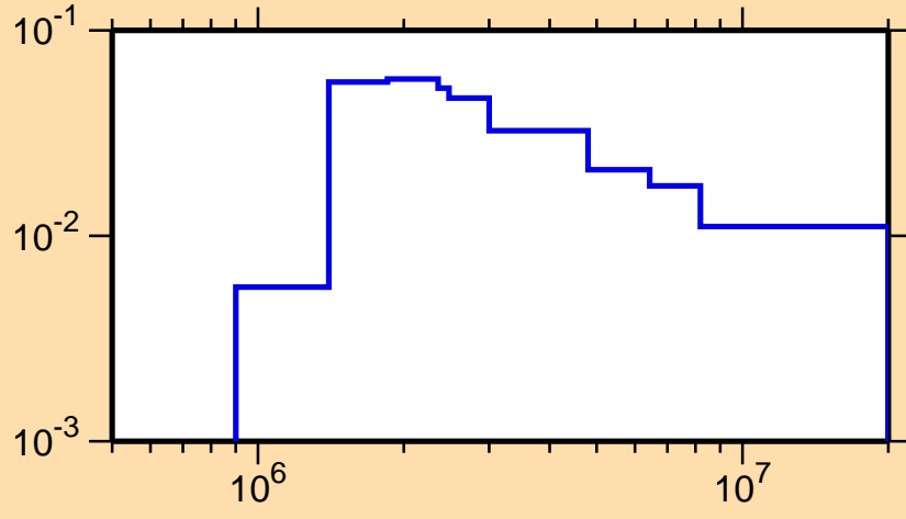
\sigma vs. E for ^{99}\text{Cd}(n,n_2)
