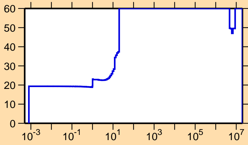
\Delta\sigma/\sigma vs. E for ^{101}\text{Cd}(n,\gamma)
