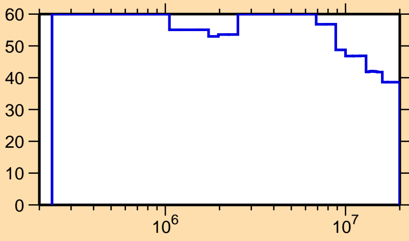
\Delta\sigma/\sigma vs. E for ^{101}\text{Cd}(n,n_1)
