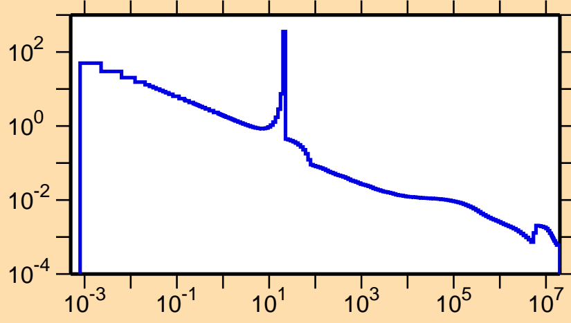
\sigma vs. E for ^{101}\text{Cd}(n,\gamma)
