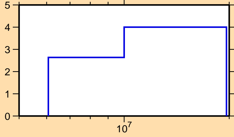
Δσ/σ vs. E for ^{101}\text{Cd}(n,\text{nonel.})
