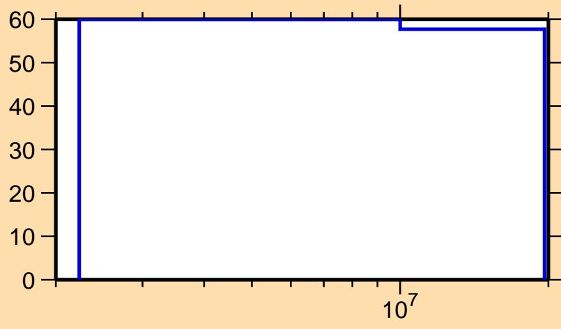
\Delta\sigma/\sigma vs. E for ^{101}\text{Cd}(n,n\text{cont.})
