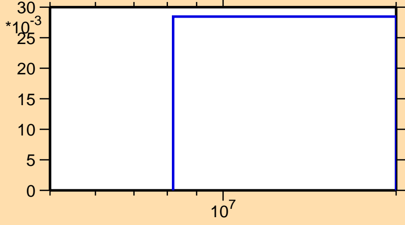
\sigma vs. E for ^{101}\text{Cd}(n,2n)
