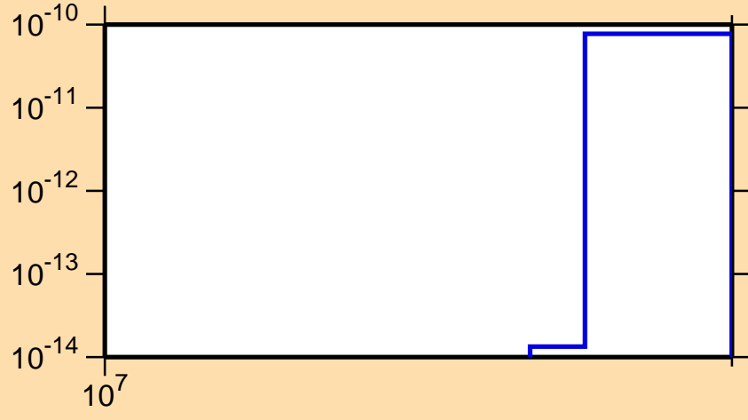
\sigma vs. E for ^{102}\text{Cd}(\text{mt } 34)
