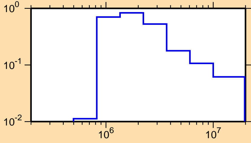
\sigma vs. E for ^{102}\text{Cd}(n,n_1)
