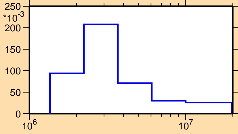
\sigma vs. E for ^{102}\text{Cd}(n,n_3)
