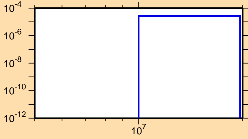
\sigma vs. E for ^{102}\text{Cd}(n,pd)
