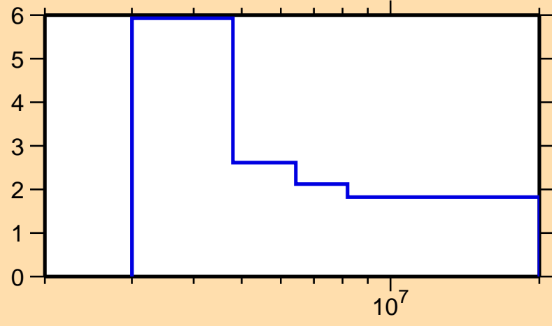
\Delta\sigma/\sigma vs. E for ^{102}\text{Cd}(n,n\text{onel.})
