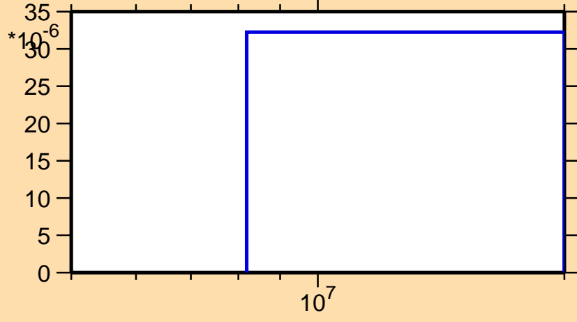
\sigma vs. E for ^{102}\text{Cd}(n,t)
