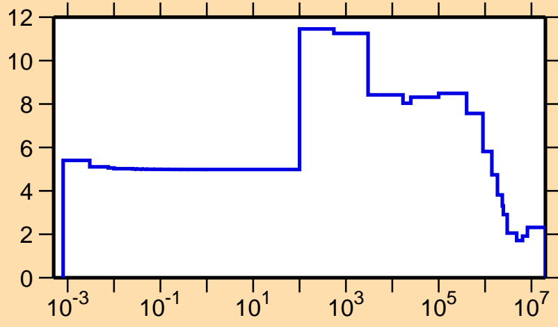
\sigma vs. E for ^{102}\text{Cd}(n,\text{el.})
