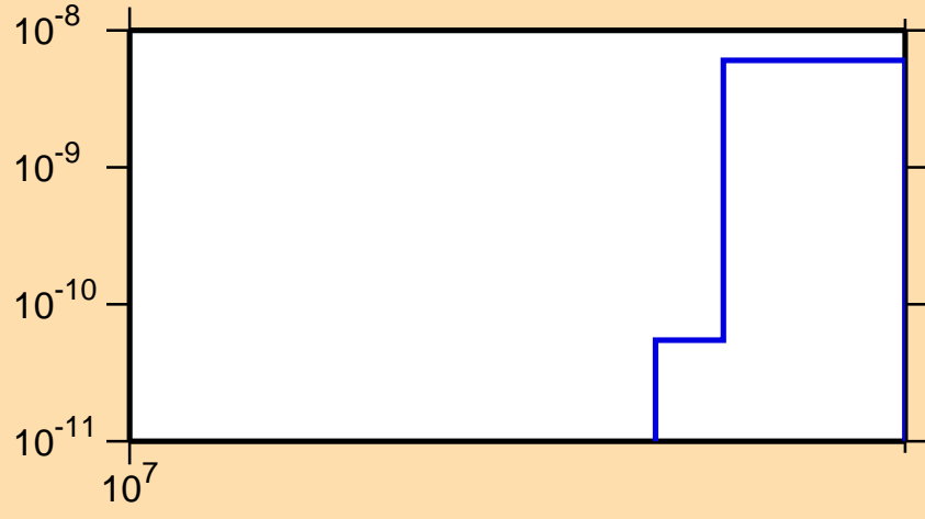
\sigma vs. E for ^{103}\text{Cd} (mt 34)
