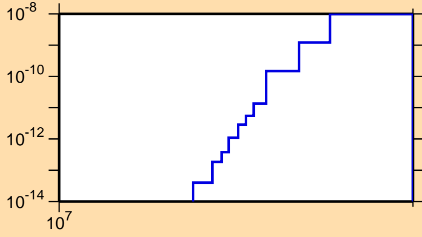
\sigma vs. E for ^{103}\text{Cd}(\text{mt117})
