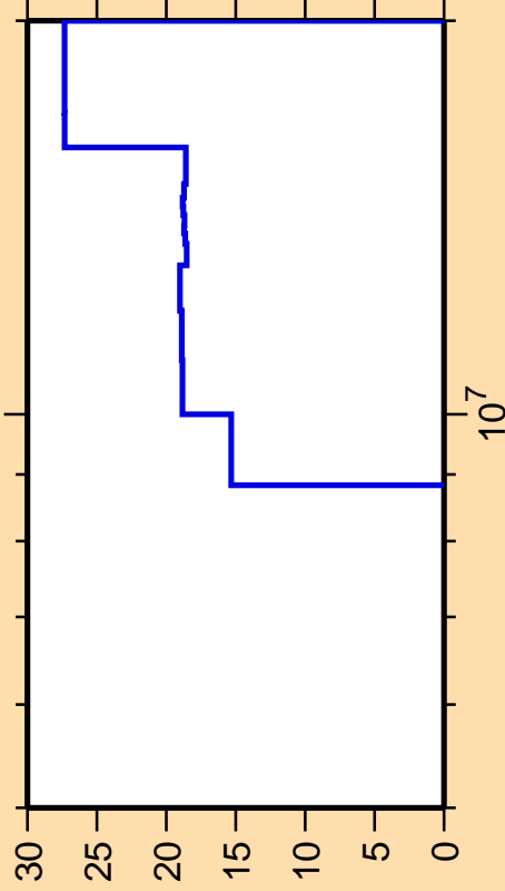
\Delta\sigma/\sigma vs. E for ^{103}\text{Cd}(n,p)
