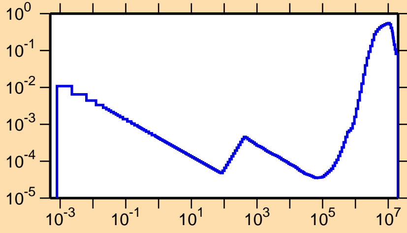
\sigma vs. E for ^{104}\text{Cd}(n,p)
