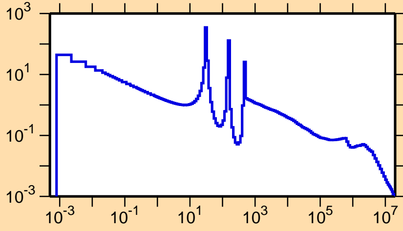
\sigma vs. E for ^{104}\text{Cd}(n,\gamma)
