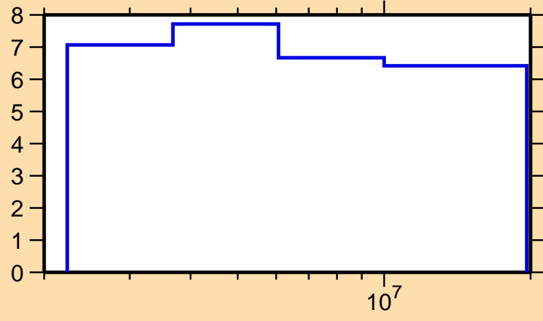
\Delta\sigma/\sigma vs. E for ^{108}\text{Cd}(n,n\text{onel.})
