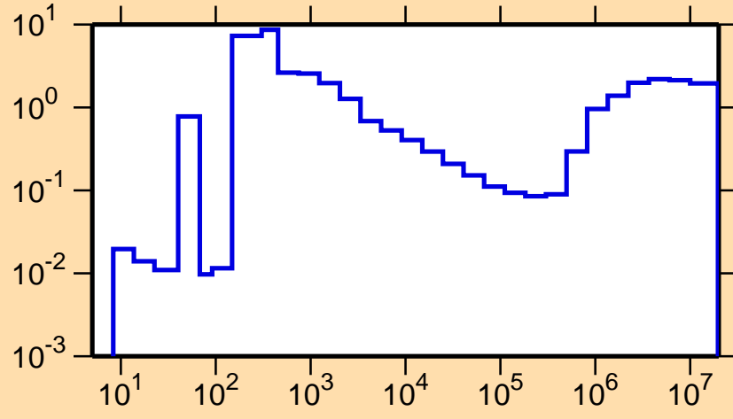
\sigma vs. E for ^{108}\text{Cd}(n,\text{nonel.})
