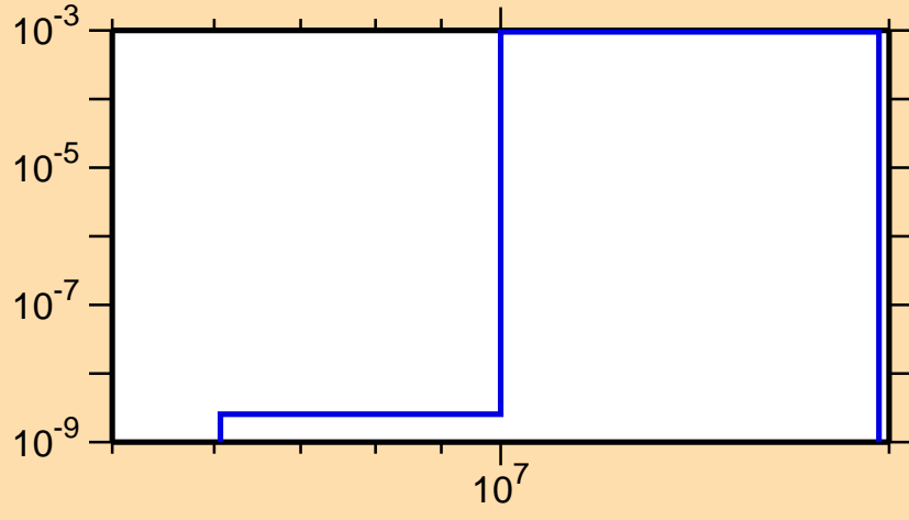
\sigma vs. E for ^{108}\text{Cd}(n,d)
