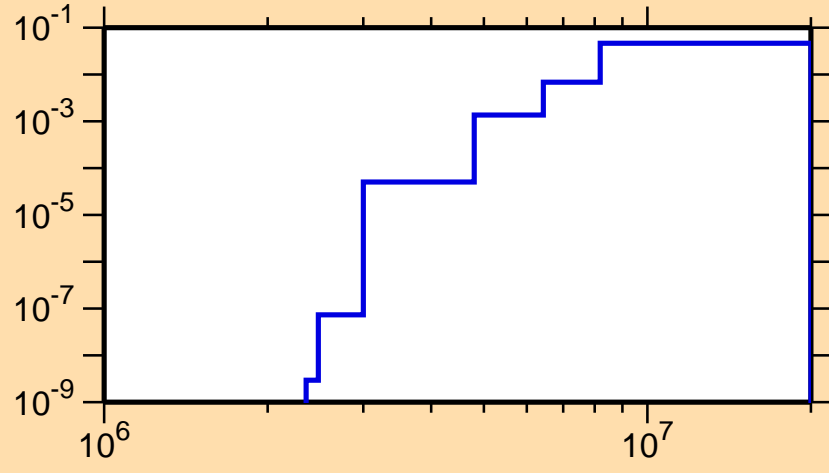
\sigma vs. E for ^{108}\text{Cd}(n,p)
