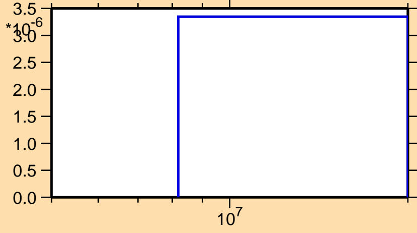
\sigma vs. E for ^{108}\text{Cd}(n,t)
