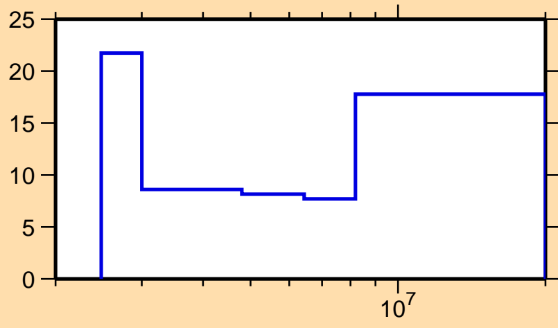
\Delta\sigma/\sigma vs. E for ^{108}\text{Cd}(n,n\text{cont.})
