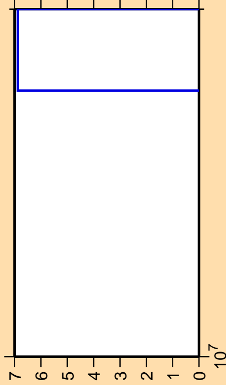
\Delta\sigma/\sigma vs. E for ^{110}\text{Cd}(n,nt)
