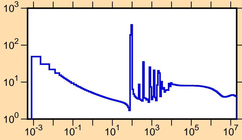
\sigma vs. E for ^{110}\text{Cd}(n,\text{tot.})
