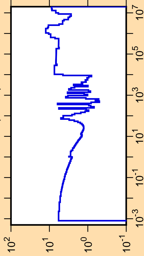
\Delta\sigma/\sigma vs. E for ^{110}\text{Cd}(n,\text{tot.})
