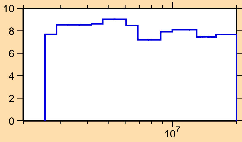
\Delta\sigma/\sigma vs. E for ^{110}\text{Cd}(n,n\text{onel.})
