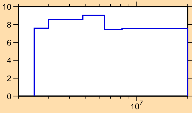
\Delta\sigma/\sigma vs. E for ^{110}\text{Cd}(n,n\text{nonel.})
