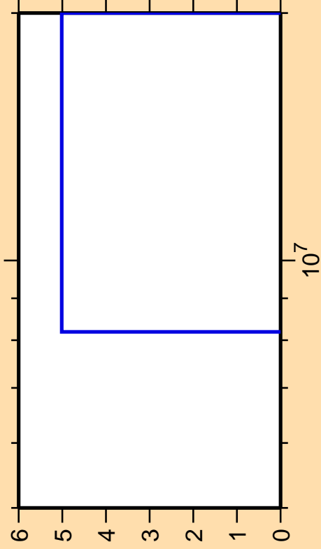
\Delta\sigma/\sigma vs. E for ^{110}\text{Cd}(n,2n\alpha)
