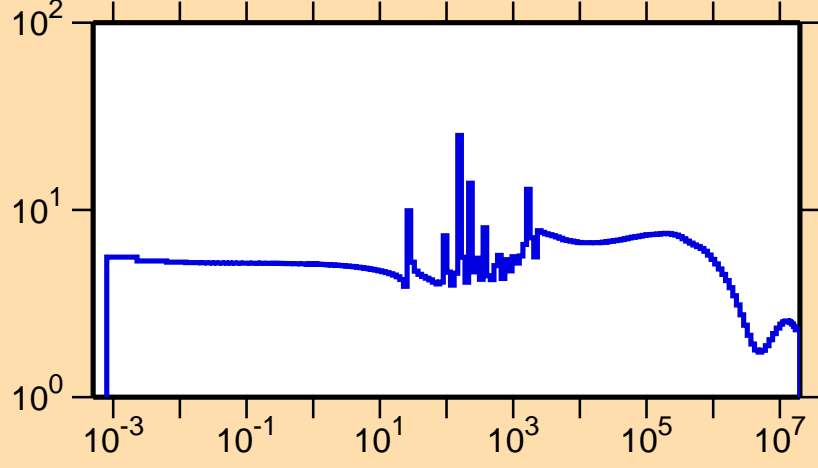
\sigma vs. E for ^{111}\text{Cd}(n,\text{el.})
