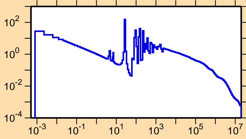
\sigma vs. E for ^{111}\text{Cd}(n,\gamma)
