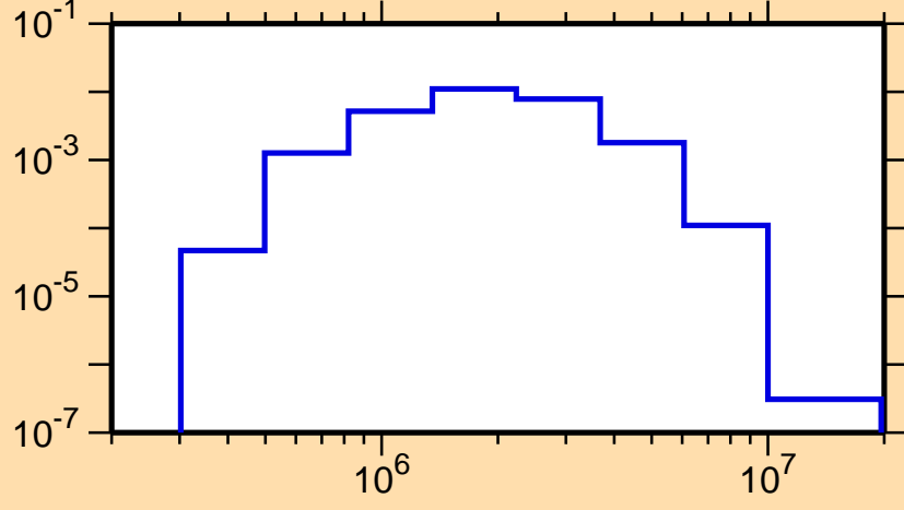
\sigma vs. E for ^{111}\text{Cd}(n,n_3)
