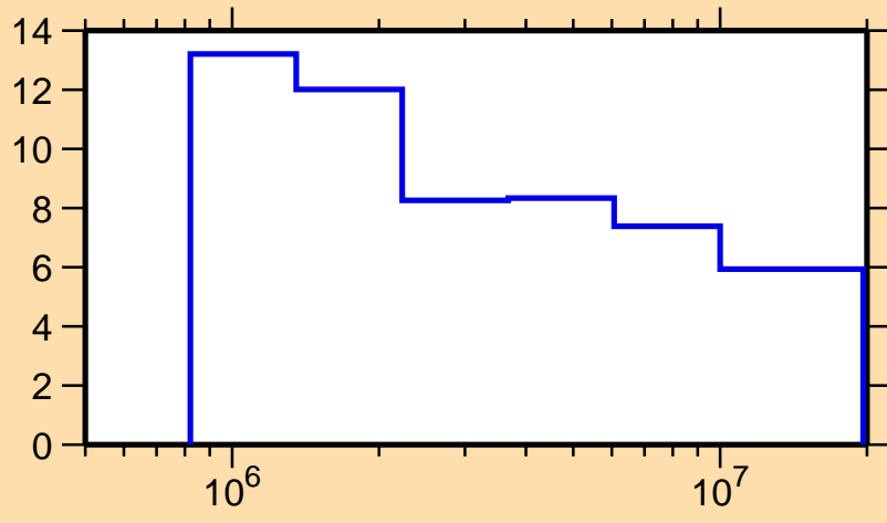
\Delta\sigma/\sigma vs. E for ^{111}\text{Cd}(n,n\text{onel.})
