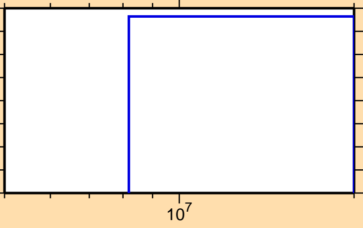
\sigma vs. E for ^{111}\text{Cd}(n,3n)
