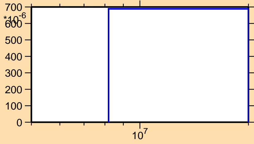
\sigma vs. E for ^{111}\text{Cd}(n,np)
