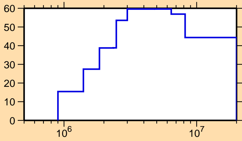
\Delta\sigma/\sigma vs. E for ^{111}\text{Cd}(n,\gamma)
