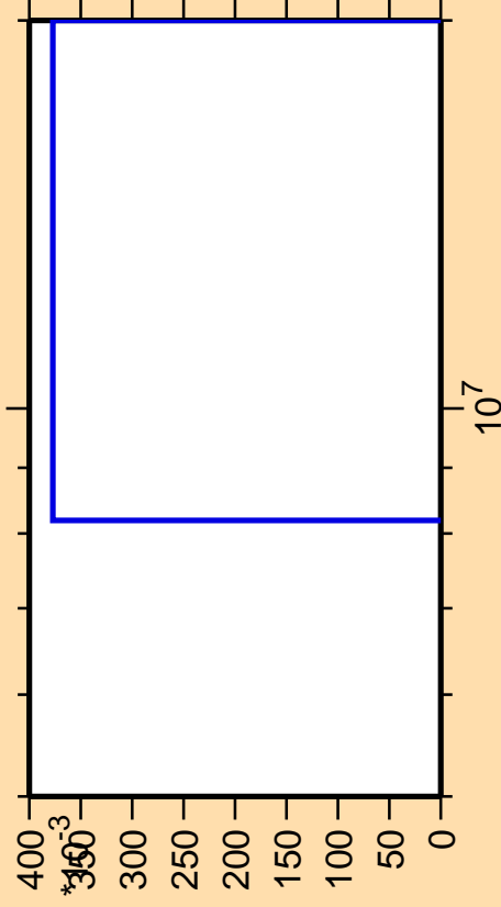
\Delta\sigma/\sigma vs. E for ^{111}\text{Cd}(n,nt)
