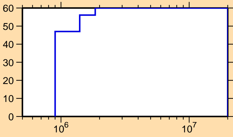
\Delta\sigma/\sigma vs. E for ^{111}\text{Cd}(n,n_1)
