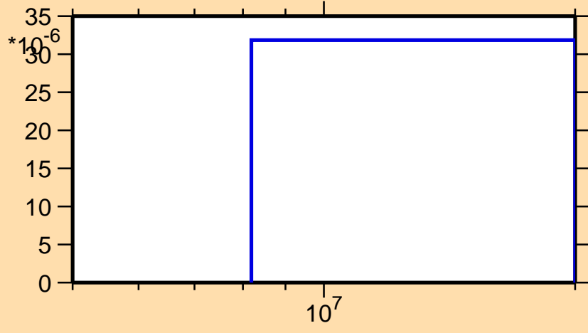
\sigma vs. E for ^{111}\text{Cd}(n,t)
