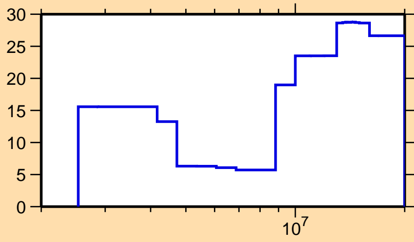
\Delta\sigma/\sigma vs. E for ^{112}\text{Cd}(n,n\text{cont.})
