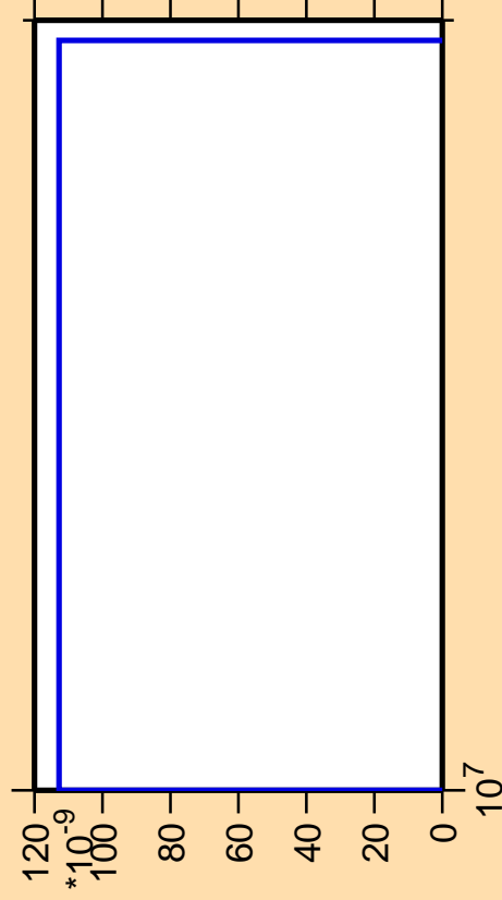
\Delta\sigma/\sigma vs. E for ^{112}\text{Cd} (mt 34)
