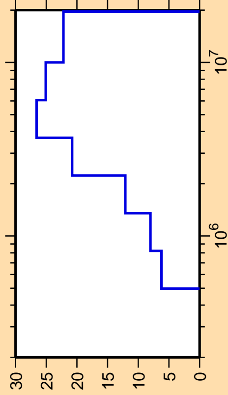
\Delta\sigma/\sigma vs. E for ^{112}\text{Cd}(n,n_1)
