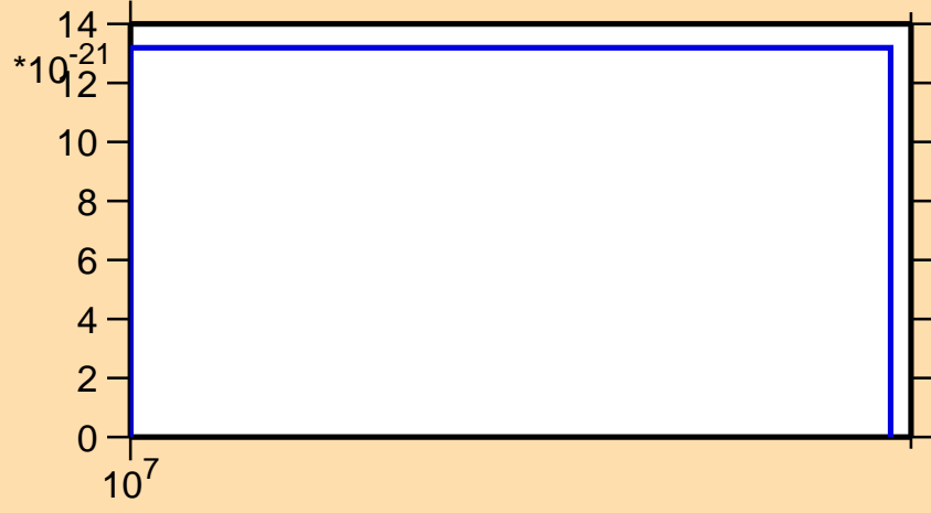
\sigma vs. E for ^{112}\text{Cd} (mt 34)
