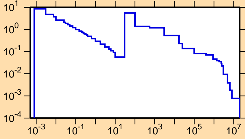
\sigma vs. E for ^{112}\text{Cd}(n,\gamma)
