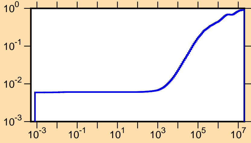
\mu vs. E for ^{114}\text{Cd}(\text{mt251})
