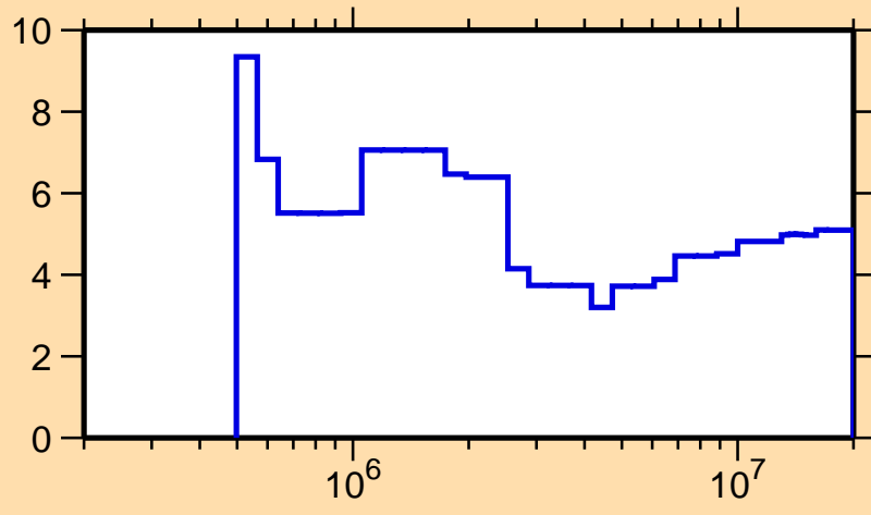
\Delta\sigma/\sigma vs. E for ^{114}\text{Cd}(n,\text{tot.})
