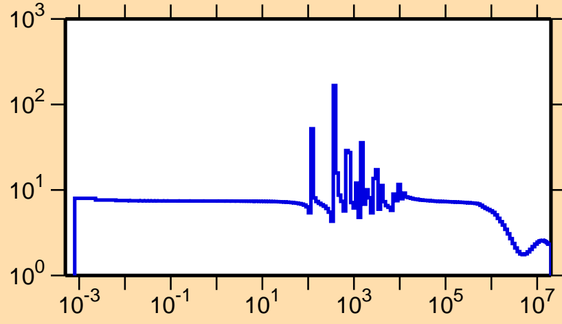
\sigma vs. E for ^{114}\text{Cd}(n,\text{el.})
