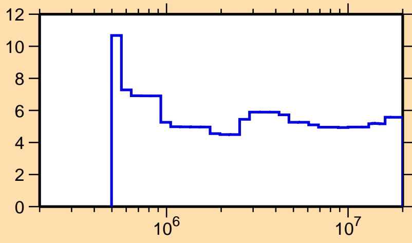
\Delta\sigma/\sigma vs. E for ^{114}\text{Cd}(n,\text{nonel.})
