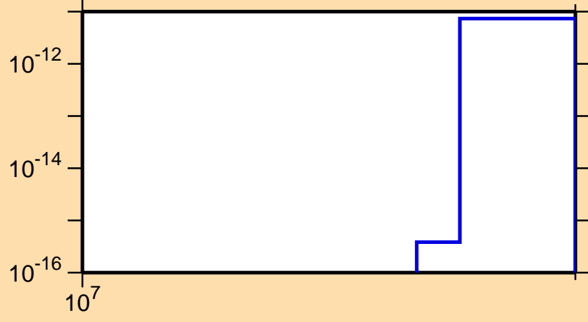
\sigma vs. E for ^{114}\text{Cd}(n,nt)
