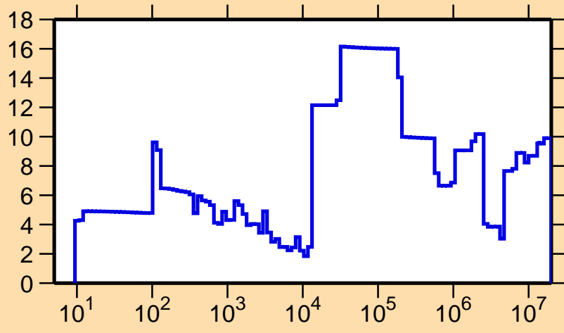
\Delta\sigma/\sigma vs. E for ^{114}\text{Cd}(n,\text{el.})
