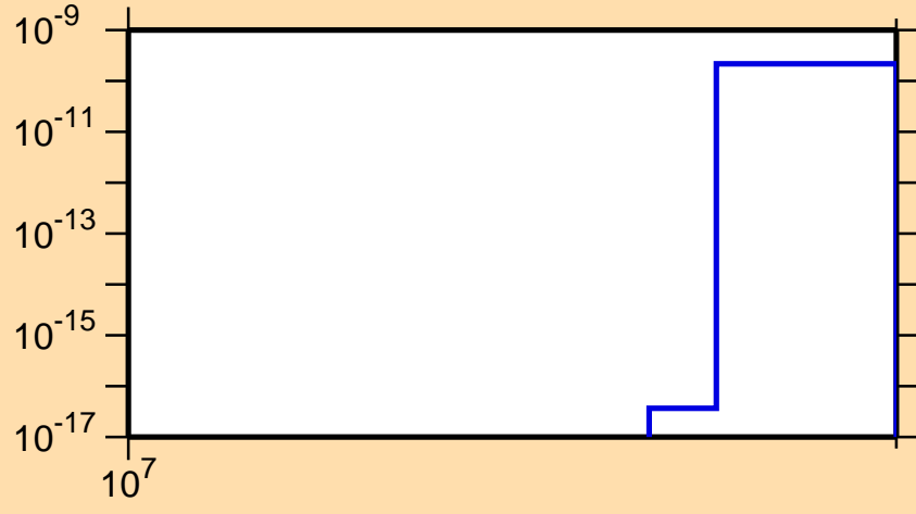
\sigma vs. E for ^{114}\text{Cd}(n,\text{nd})
