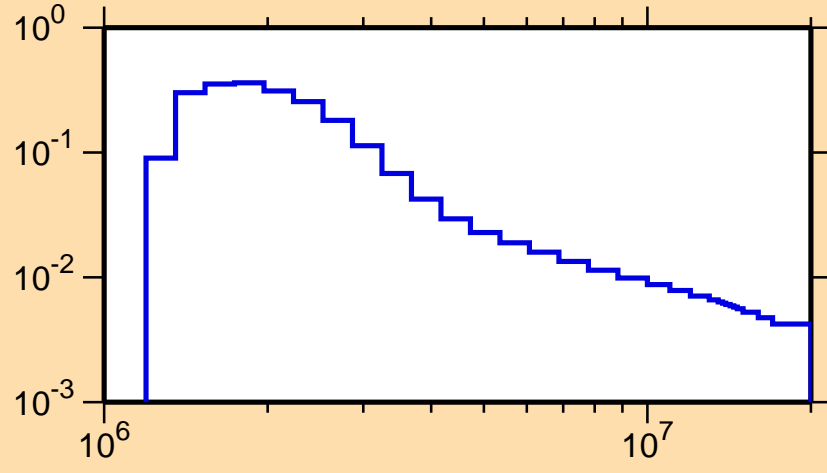
\sigma vs. E for ^{114}\text{Cd}(n,n_3)
