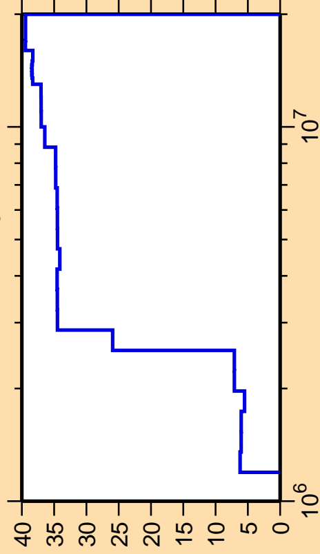
\Delta\sigma/\sigma vs. E for ^{114}\text{Cd}(n,n_3)
